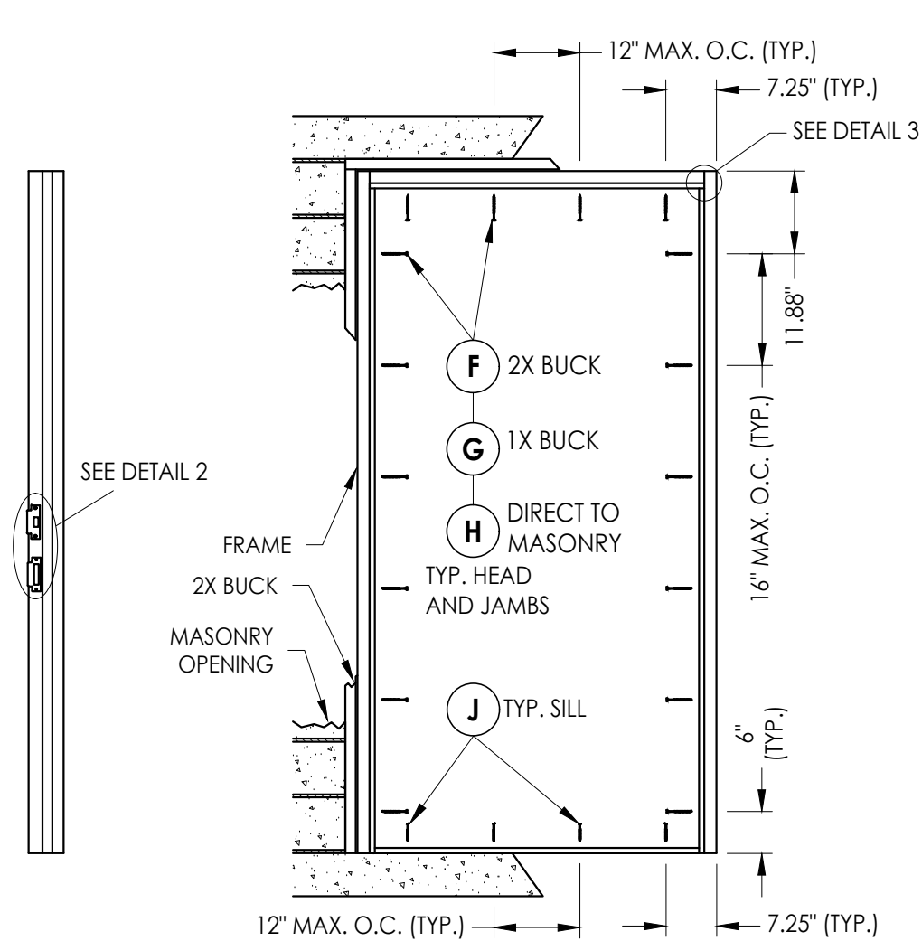
FRAME ANCHORING
