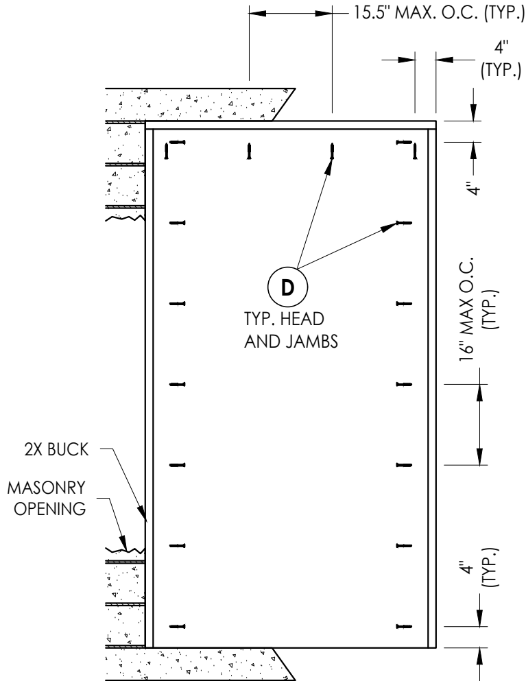
BUCK ANCHORING
