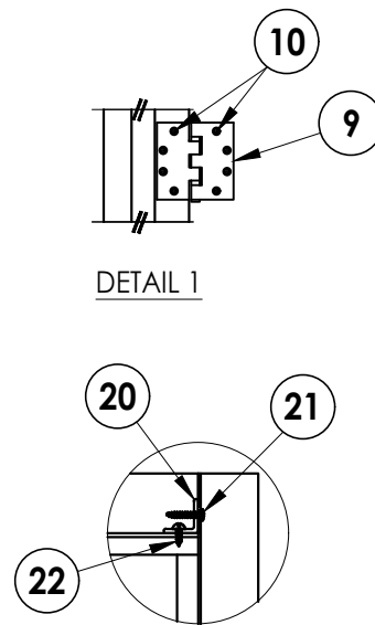
DETAIL 3
