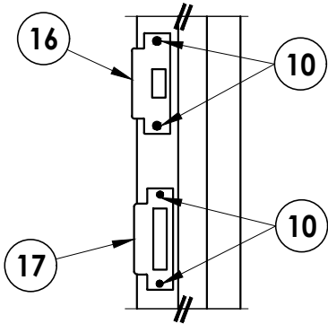
DETAIL 1 LOCK & DEADBOLT
